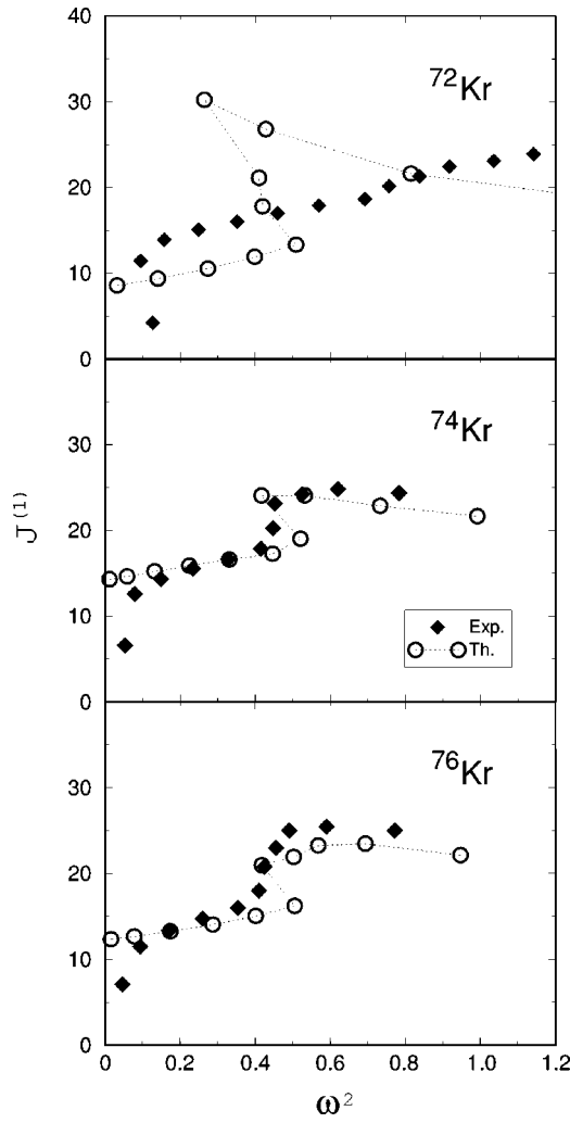
FIG. 1. Moments of inertia \mathcal{J}^{(1)} = \{(2I-1)/[E(I)-E(I-2)]\} ( \hbar^2/\text{MeV} ) as function of \omega^2 with \omega = \{[E(I)-E(I-2)]/2\} ( \text{MeV}/\hbar ). Theoretical results with the standard interaction in the PSM are compared with the experimental data. The experimental data are taken from Ref. [1] for ^{72}\text{Kr} , Ref. [4] for ^{74}\text{Kr} , and Ref. [11] for ^{76}\text{Kr} .
