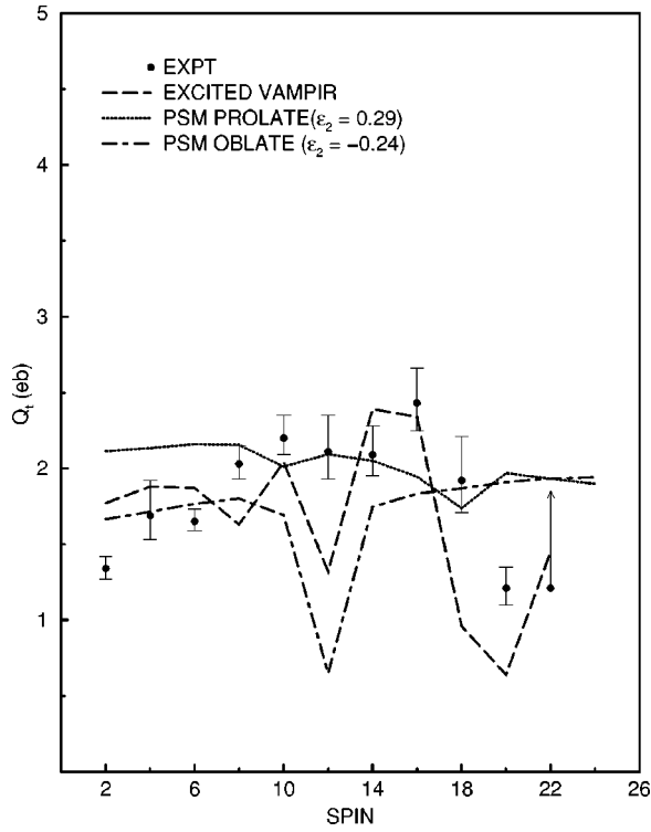
FIG. 4. Comparison of the measured transition quadrupole moments Q_t for excited states in ^{72}\text{Se} with the predictions of PSM and EXCITED VAMPIR model. The PSM is calculated with a prolate shape \epsilon_2 = 0.29 and an oblate shape \epsilon_2 = -0.24 .
