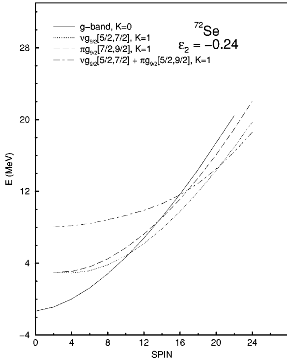
FIG. 5. Band diagram of ^{72}\text{Se} for an oblate shape with \epsilon_2 = -0.24 .
