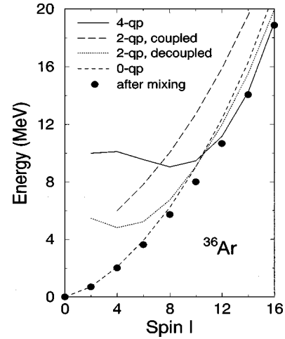
FIG. 1. Band diagram (bands before configuration mixing) and the yrast band (the lowest band after configuration mixing, denoted by dots) for the superdeformed nucleus ^{36}\text{Ar} . Only the important lowest-lying bands in each configuration are shown.
